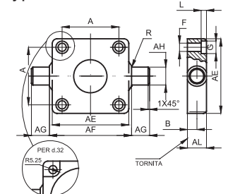
Centre trunnion (tie rod) for heads
