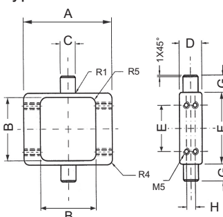
Centre trunnion (tie rod) for cylinders AMC
